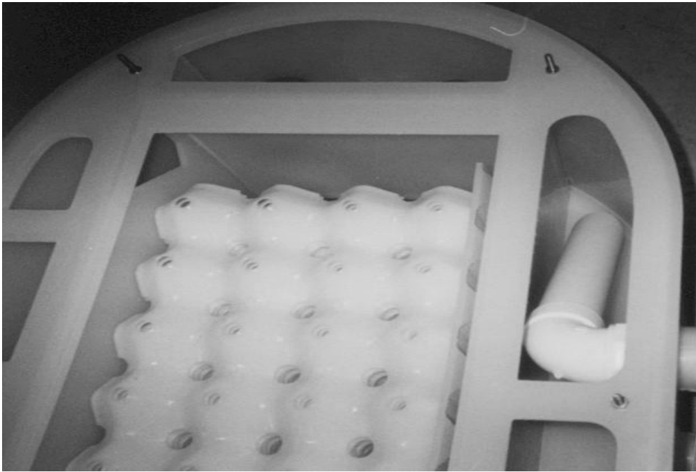
MSR 11 view looking toward outlet. Inlet distributor and plates can be seen as well as oil overflow v-weir and plate seals.
