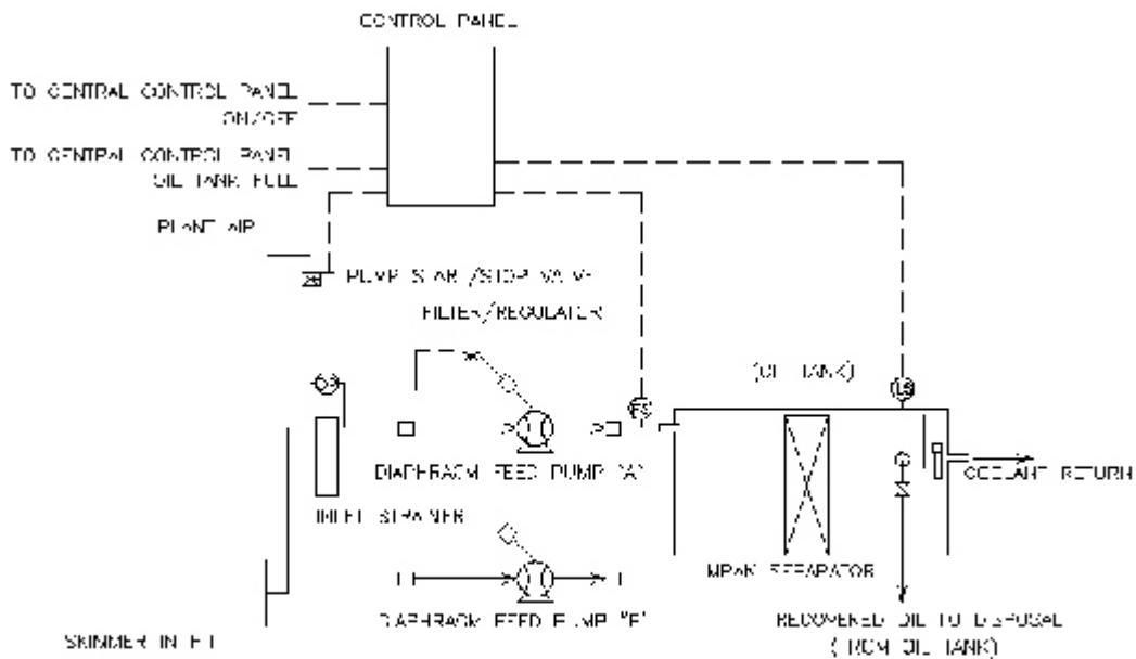
FIGURE 2 SEPARATOR SYSTEM SCHEMATIC
