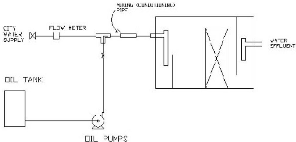
Figure 3. Schematic of Flows During Test
