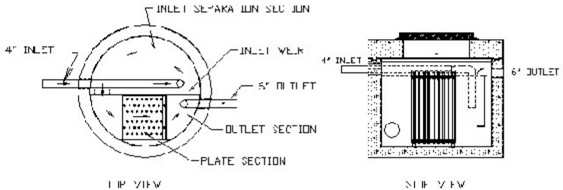
Figure 2: Stormwater Separator
